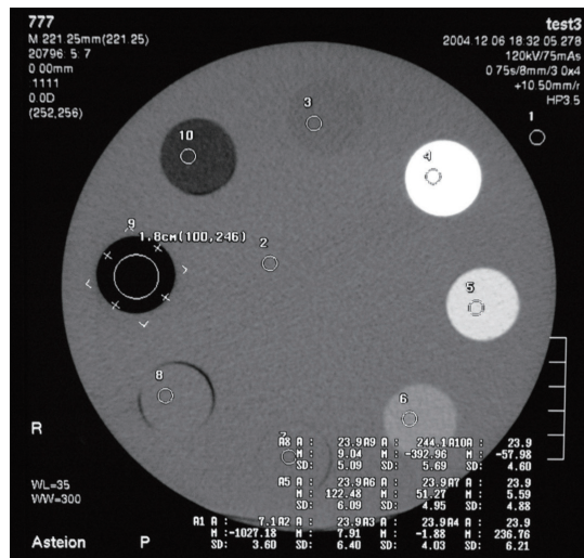
linearity phantom
